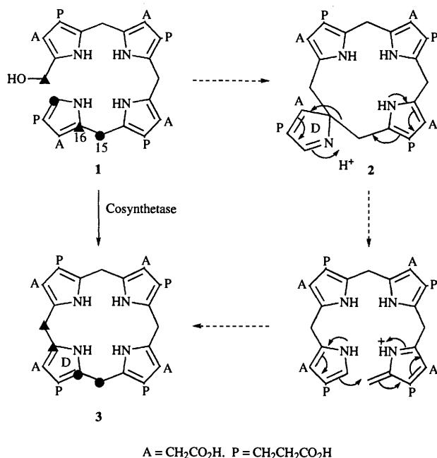
Scheme 1 Proposed mechanism for the formation of uro'gen III by cosynthetase
