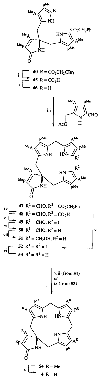
Scheme 5 Reagents: i, Zn, AcOH; ii, \text{CF}_3\text{CO}_2\text{H} ; iii, \text{SnCl}_4 ; iv, \text{H}_2/\text{Pd} ; v, \text{KI}_3 , \text{NaHCO}_3 ; vi, \text{H}_2/\text{Pt} ; vii, \text{NaBH}_4 ; viii, TsOH; ix, \text{CH}_2\text{O} , \text{CF}_3\text{CO}_2\text{H} ; x, KOH, \text{H}_2\text{O} , MeOH
