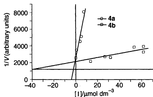
Fig. 3 Dixon plot for the inhibition of cosynthetase by the enantiomeric spiro lactams 4a and 4b . The horizontal line at 1/V = 1218 is at 1/V_{\max} and the straight lines through the experimental points intersect it at [I] = -K_i .
