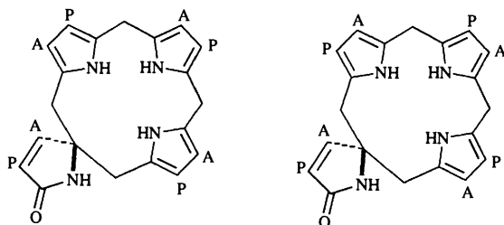
Fig. 4 The two enantiomers of the spiro lactam 4
