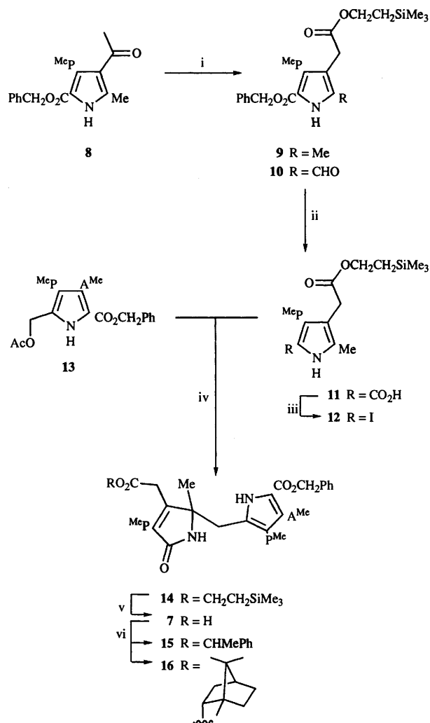
Scheme 2 Reagents: i, \text{Tl}(\text{NO}_3)_3 \cdot 3\text{H}_2\text{O} , \text{HNO}_3 , \text{Me}_3\text{SiCH}_2\text{CH}_2\text{OH} ; ii, \text{H}_2/\text{Pd} ; iii, \text{KI}_3 , \text{NaHCO}_3 ; iv, \text{SnCl}_4 then \text{AgOAc} , \text{TsOH} , \text{H}_2\text{O} ; v, \text{TBAF} ; vi, \text{DCC} , \text{DMAP} , \text{ROH}
