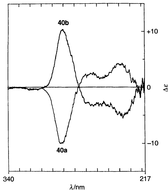
Fig. 2 Circular dichroism spectra of the enantiomers 40a derived from peak X (Fig. 1) and 40b derived from peak Y
